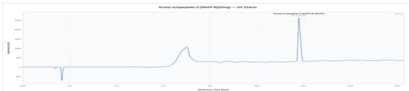
SNAP-8 10mg - SOL-SNAP8-10MG: UV Chromatogram
