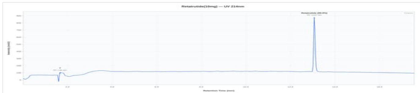
GLP-RT 10mg 10mg - SOL-SC10mg: UV Chromatogram
