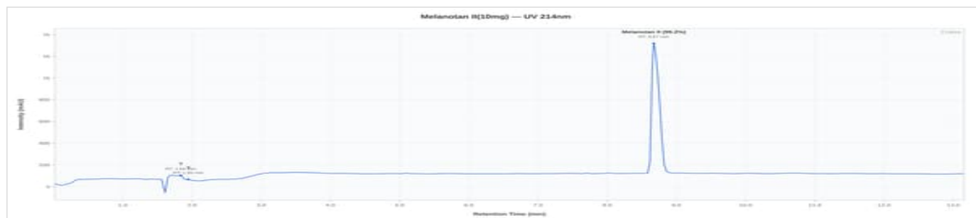
Melanotan II 10mg 10mg - SOL-MT210mg: UV Chromatogram
