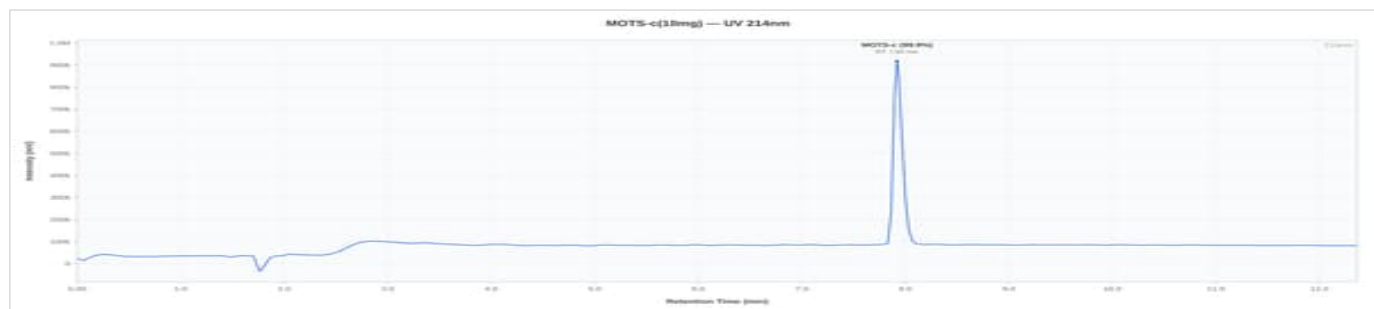
MOTS-C 10mg 10mg - SOL-MS10: UV Chromatogram
