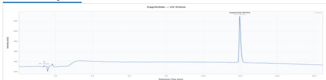
Cagrilintide 10mg 10mg - 1: UV Chromatogram
