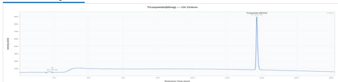
Trizepatide 60mg - 061926: UV Chromatogram
